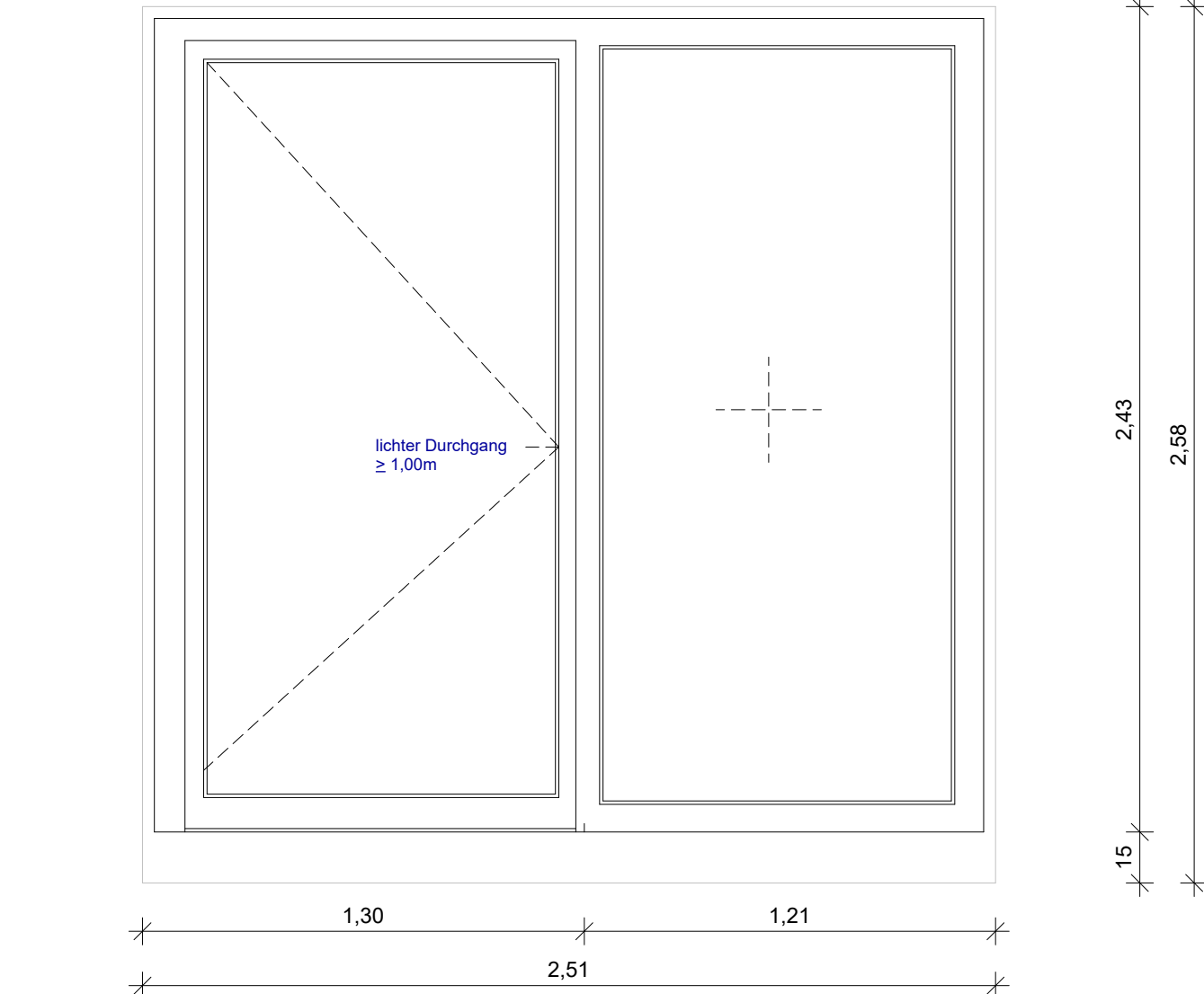
POS. 1.2.40 MEI-4 Aluminium-Brandschutz-Element RS
