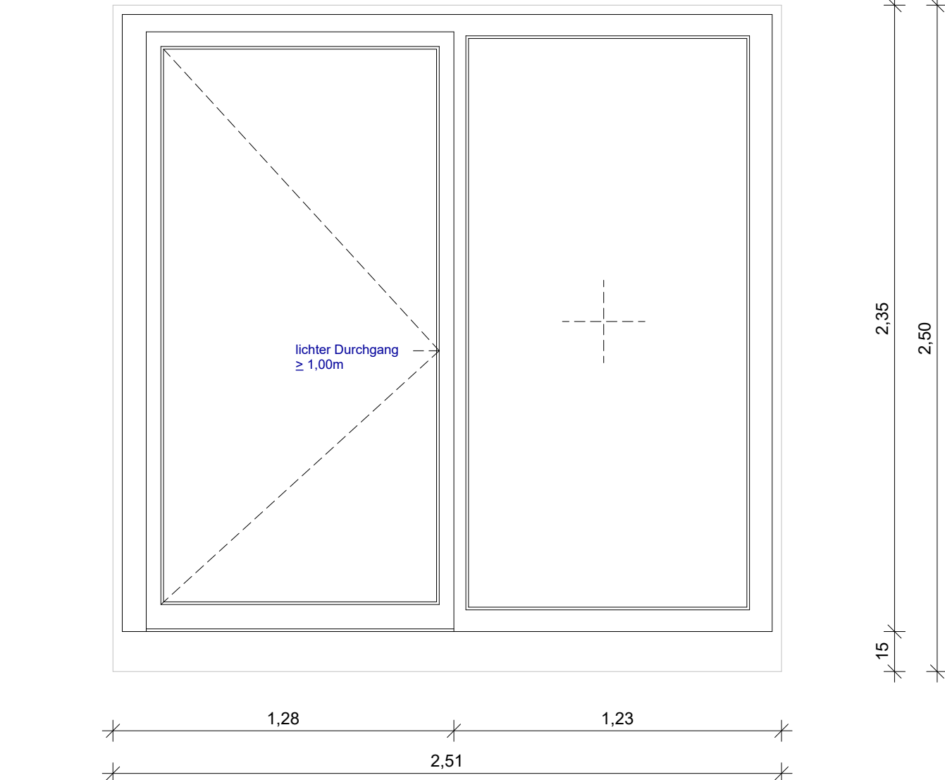
POS. 1.2.20 MEI-2 Aluminium-Brandschutz-Element RS
