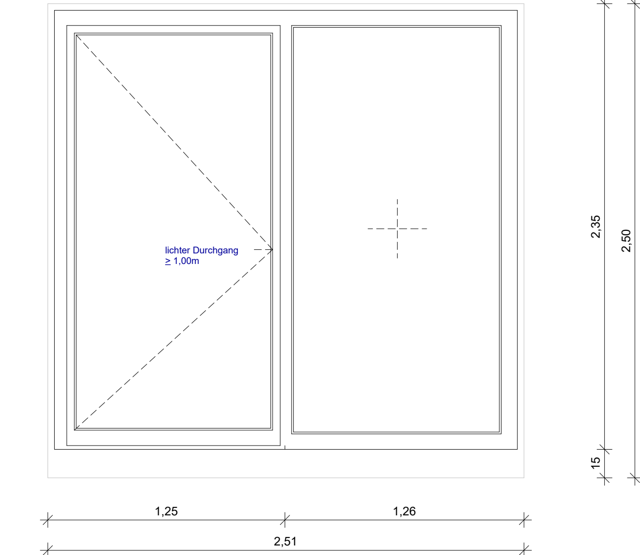
POS. 1.2.10 MEI-1 Aluminium-Brandschutz-Element RS
