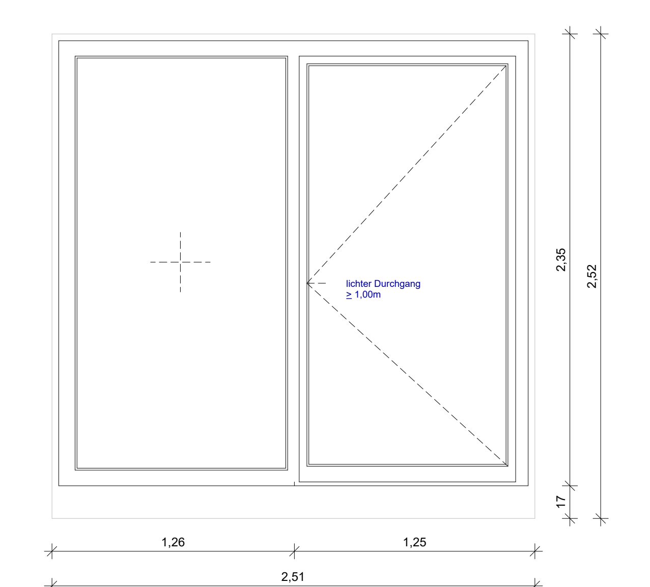
POS. 1.2.70 MEI-7 Aluminium-Brandschutz-Element RS
