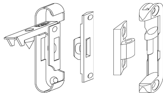
Connected window hardware, 8 sets Maco 101252 + 101251
