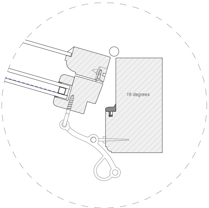
Opening position Roca 911341 storm hook 2nd position
