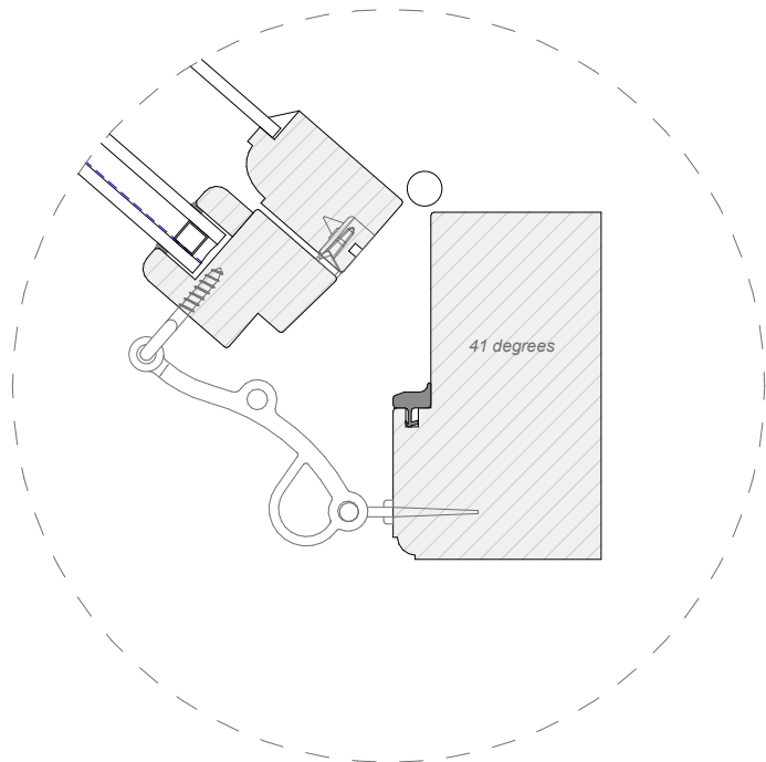
Opening position Roca 911341 storm hook 1st position
